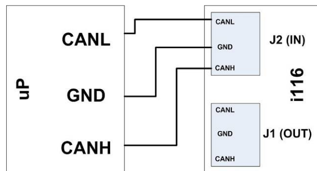
Figure 4: CAN interface connection
