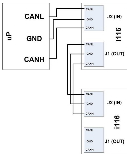
Figure 5: Multiple node connection
