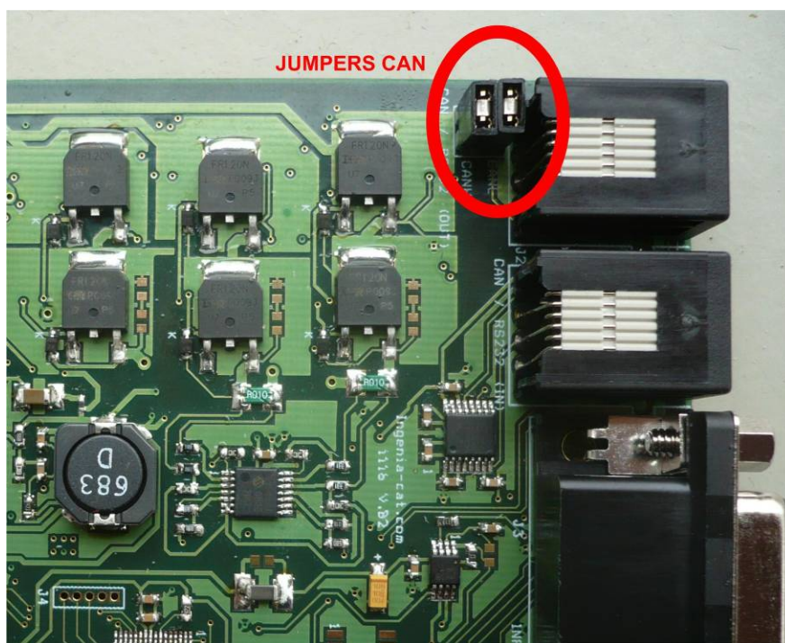
Figure 6: For CAN communications, jumpers must be placed
