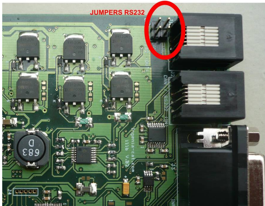
Figure 9: For RS232 communications, jumpers must be taken off
